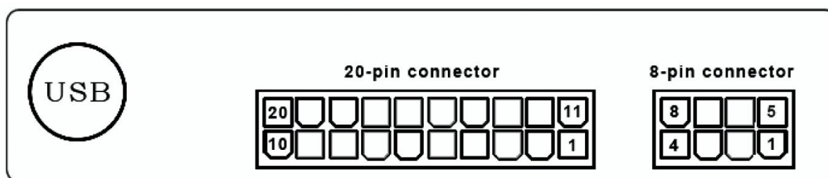
Figure 1 - Front view of the module panel
