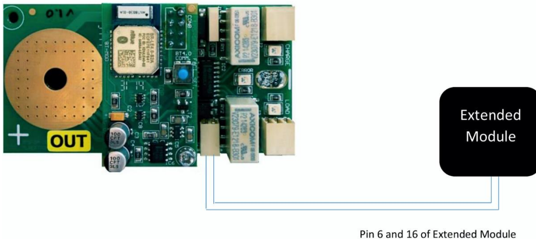
Figure 3 – Connecting the OUT module with the Extended Module
